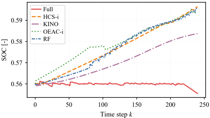
B001, I010_L1_v11_SOC056
