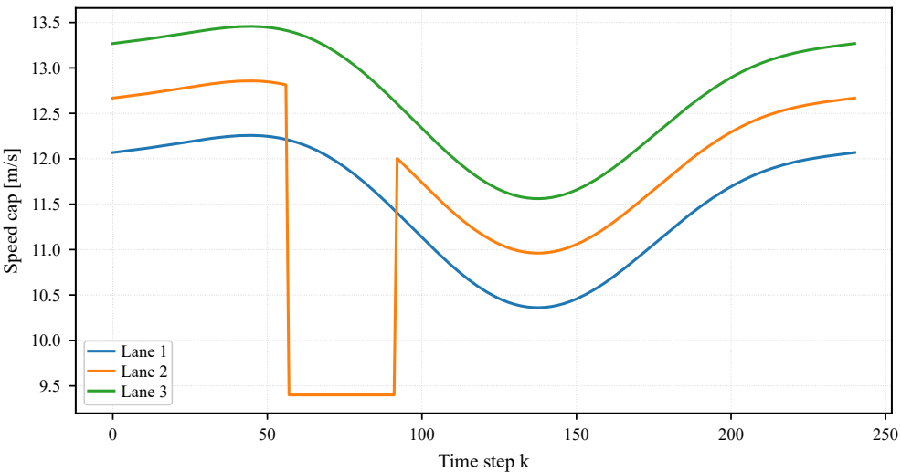
B010: speed-cap profiles
