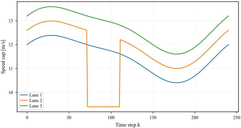
B003: speed-cap profiles
