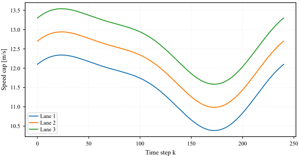
B004: speed-cap profiles
