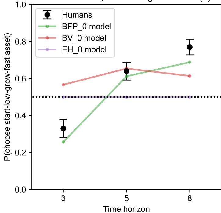
A Fitted models, without logistic offset (b)
