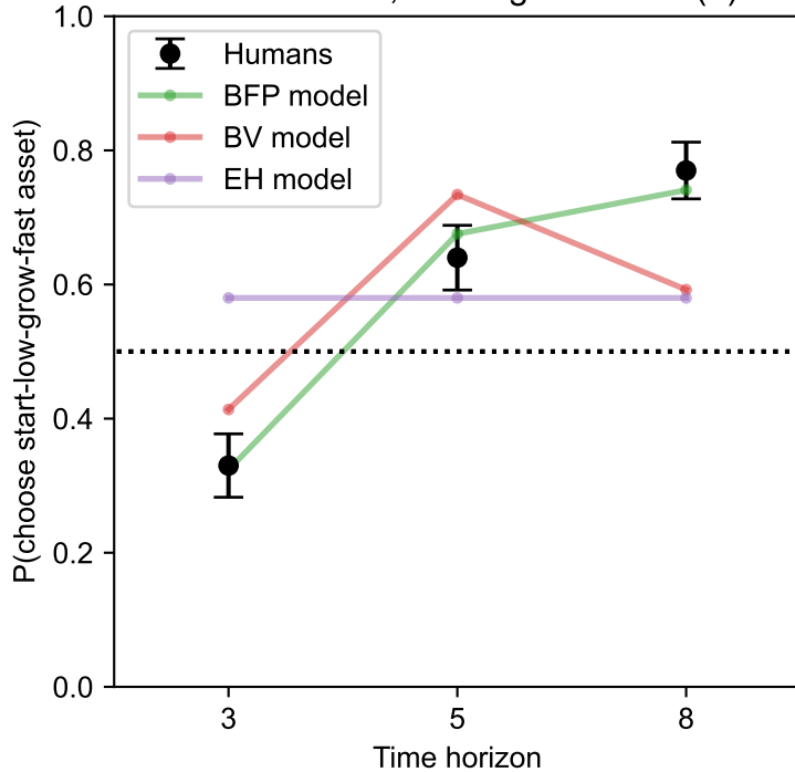
B Fitted models, with logistic offset (b)
