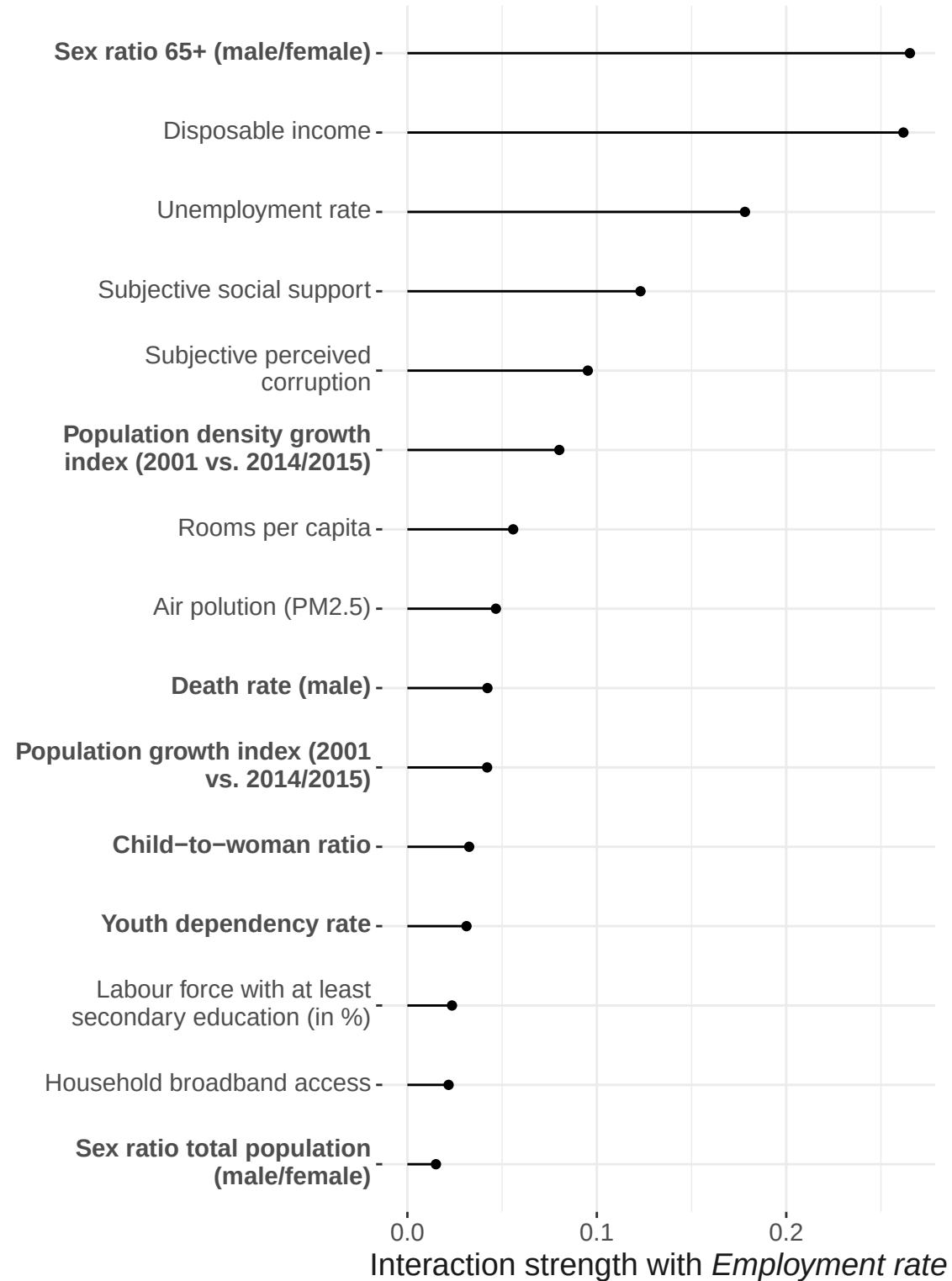
XGBoost
