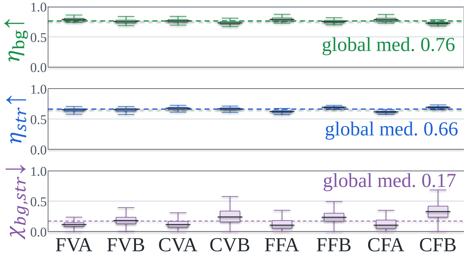
(b) Role specialization diagnostics
