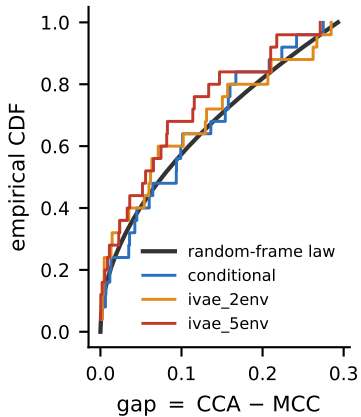
(a) no arm rejects the null
