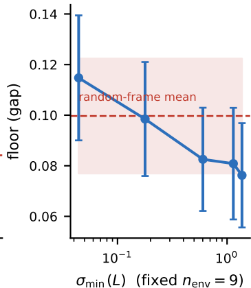
(c) monotone, but never rejects
