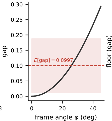
(b) gap = 1 - \cos \varphi
