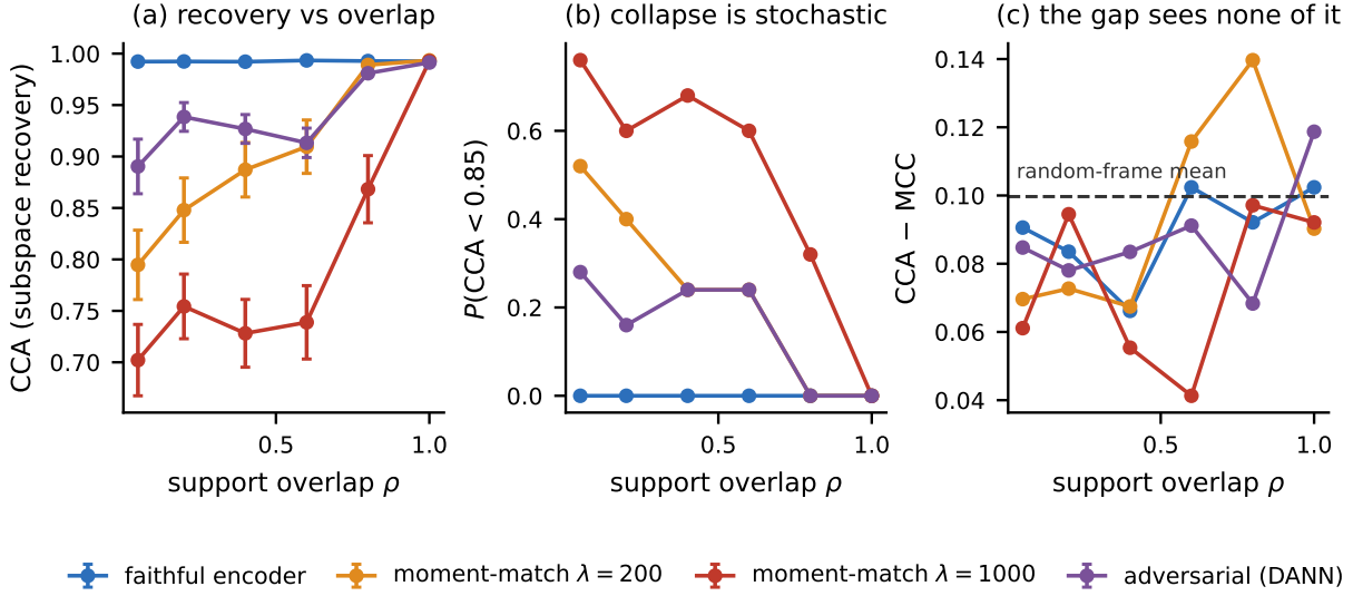
Figure 4: (a) A faithful per-sample encoder is flat in \rho ; alignment objectives collapse. (b) The collapse is stochastic. (c) \text{CCA} - \text{MCC} sits on the random-frame mean throughout and is blind to the effect in (a), because the folding is approximately axis-factorised.
