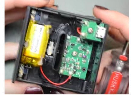
Bottom view of unfolded circuit board
