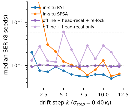
(b) common-mode drift: re-lock absorbs it
