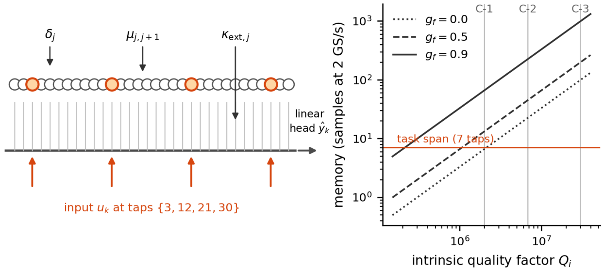
(a) trained partition \{\delta_j, \kappa_{\text{ext},j}, \mu_{j,j+1}\} , per-ring saturating gain g (b) realizable memory region
