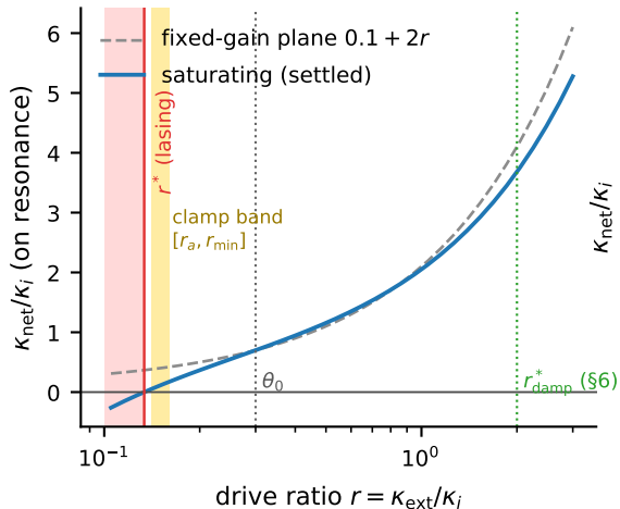
(a) operating plane and lasing clamp
