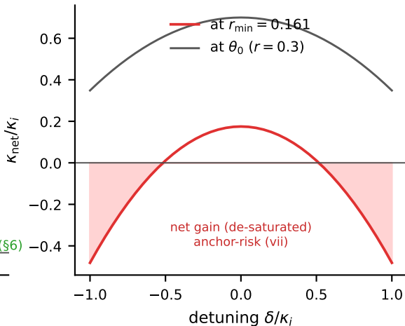
(b) off-resonance de-saturation
