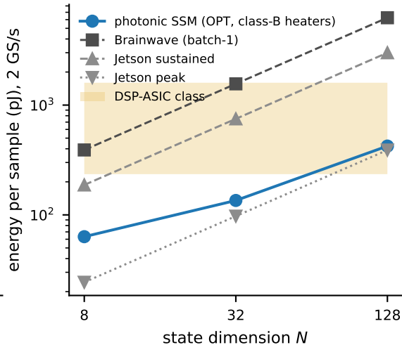
(b) inference envelope at 2 GS/s
