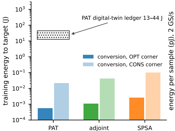
(a) training: the energy metric inverts the rank
