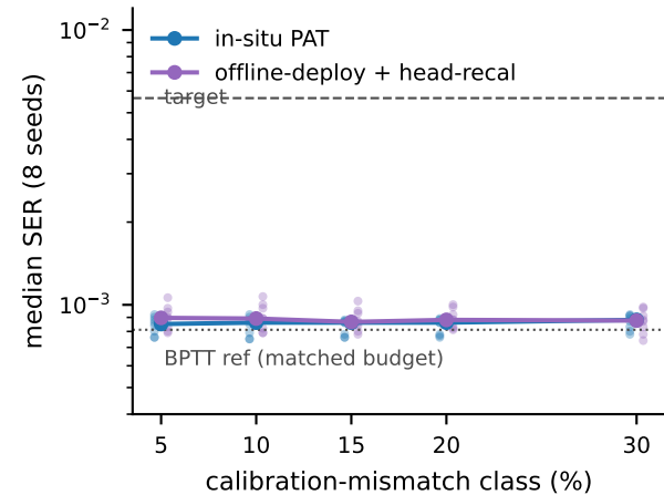
(a) corrected calibration sweep (S0.13)
