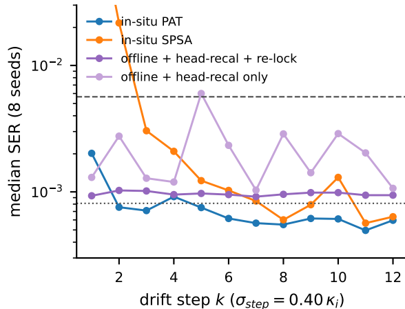
(b) common-mode drift: re-lock absorbs it
