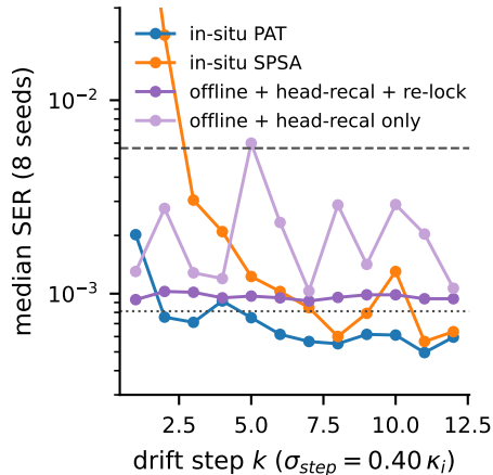
(b) common-mode drift: re-lock absorbs it
