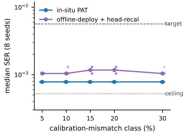
(a) tie is robust to calibration error (crossover m^* = \text{none} )
