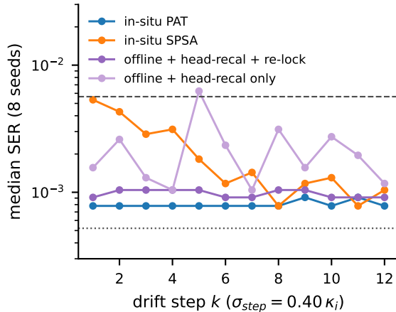
(b) common-mode drift: re-lock absorbs it
