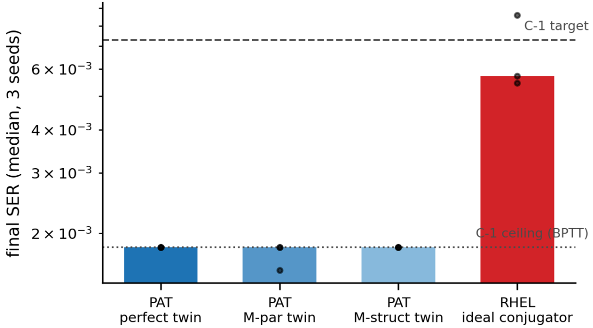
Figure S2 — Twin-mismatch decomposition at C-1 (§5.6). Final SER (3 seeds) for PAT with a perfect twin, a parametric-error (M-par) twin, and a structural-omission (M-struct) twin — all three at the C-1 BPTT ceiling, i.e. mismatch channels \approx 0 at this cell only (the dropped gain channel grows to \sim 8\% of gradient direction at C-2, §5.6) — and the idealized-conjugator RHEL control, which reaches the C-1 target and thereby localizes RHEL’s C-2 failure to echo physics, not mechanics.
