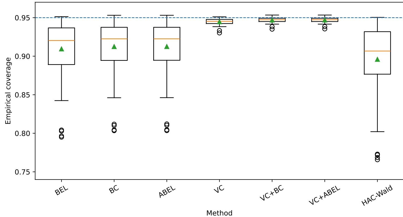
Empirical 95% coverage across 80 primary scenarios
