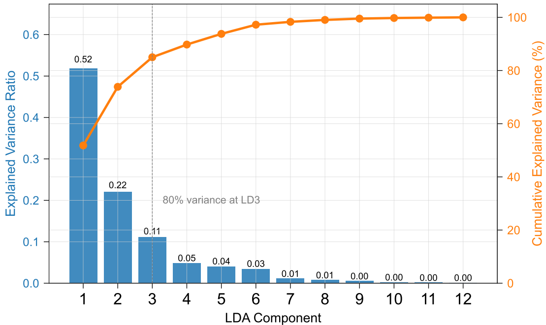
LDA Scree Plot - Variance Explained
