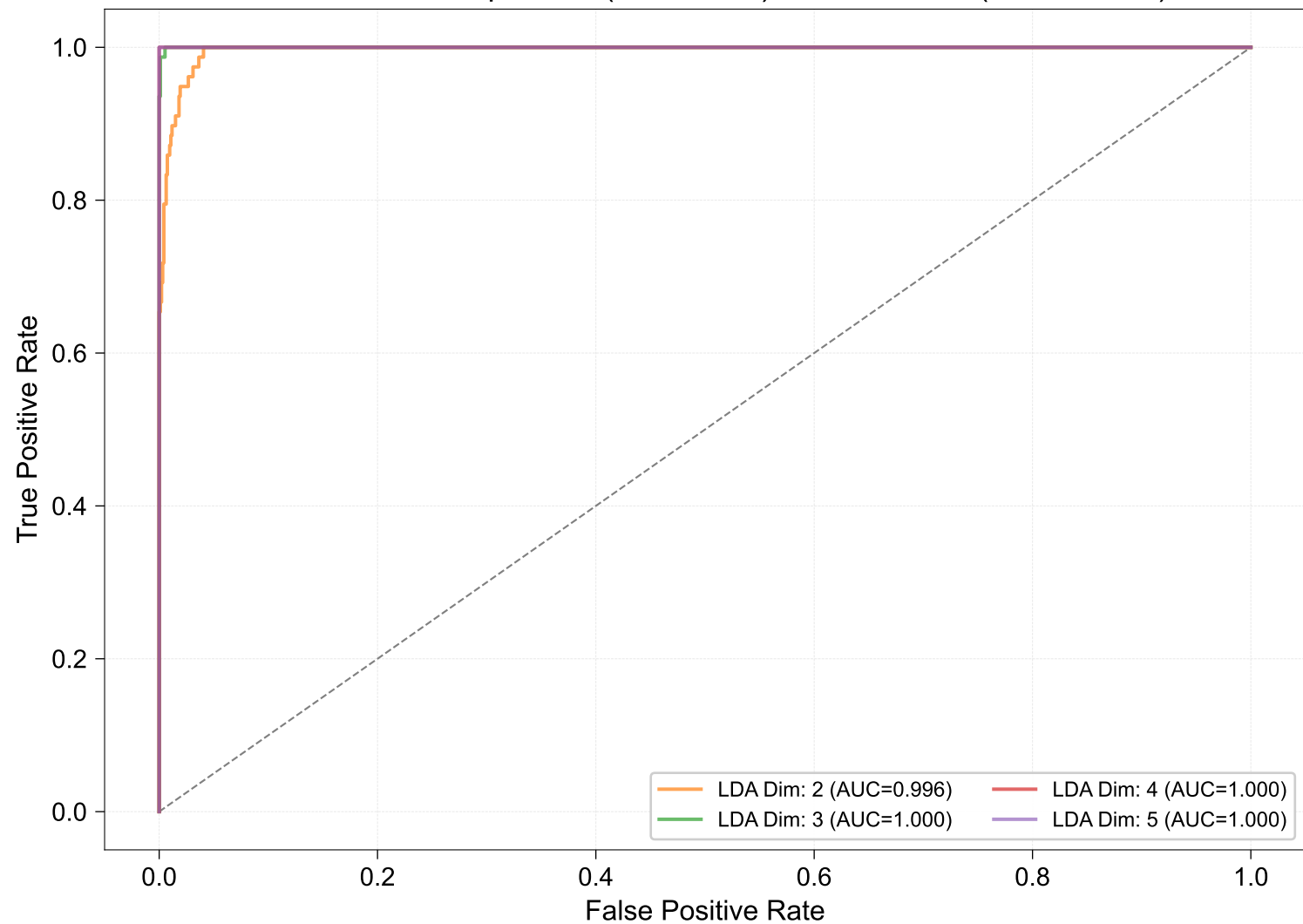
ROC Curve Comparison (5-Fold CV) - Best Dim: 4 (AUC=1.000)
