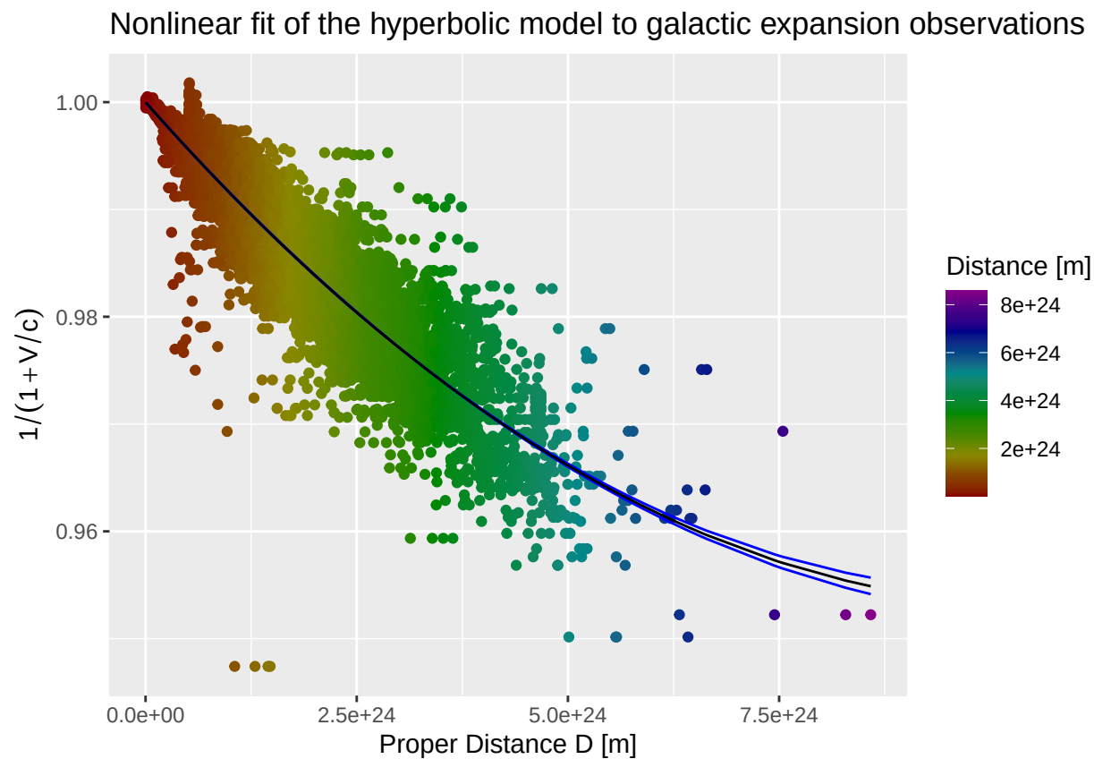
Figure 1. Fit of the hyperbolic model to the galactic distance-velocity data. The points represent the observations, and the solid line represents the nonlinear least-squares fit.
