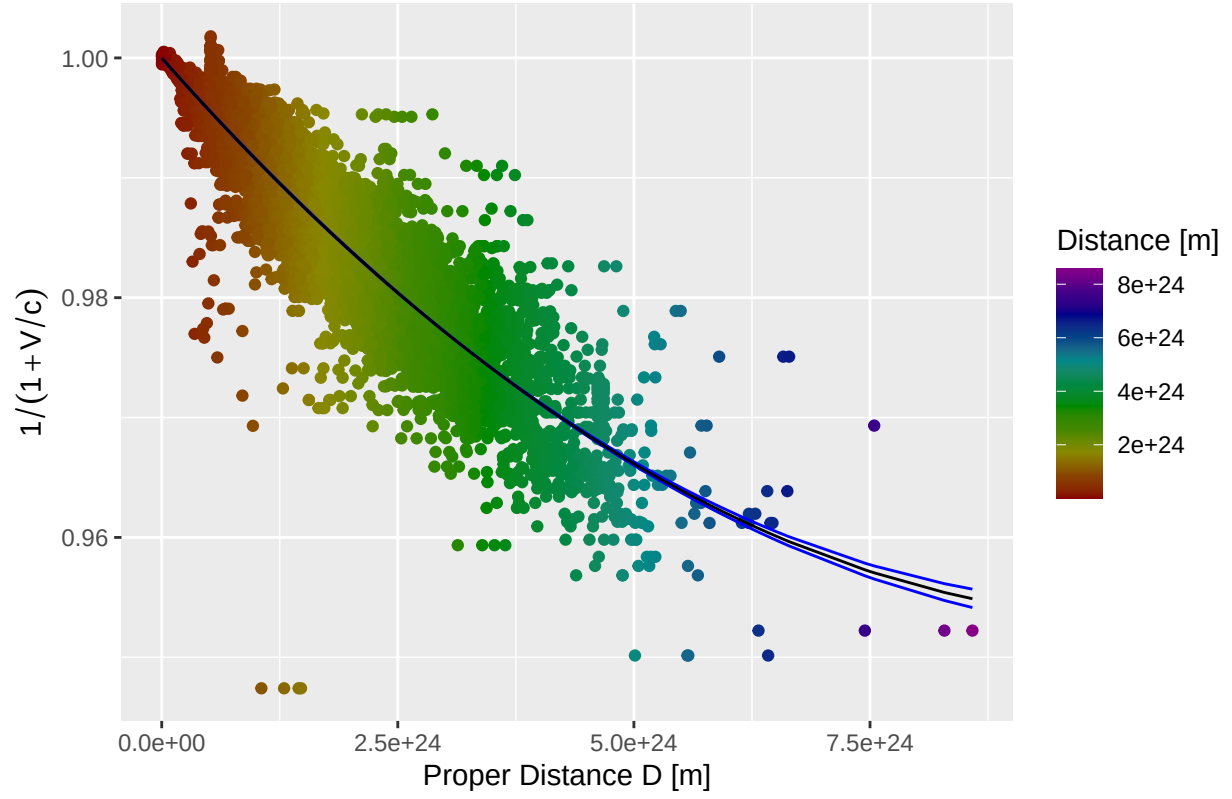
Figure 1. Fit of the hyperbolic model to the galactic distance-velocity data. The points represent the observations, and the solid line represents the nonlinear least-squares fit.
