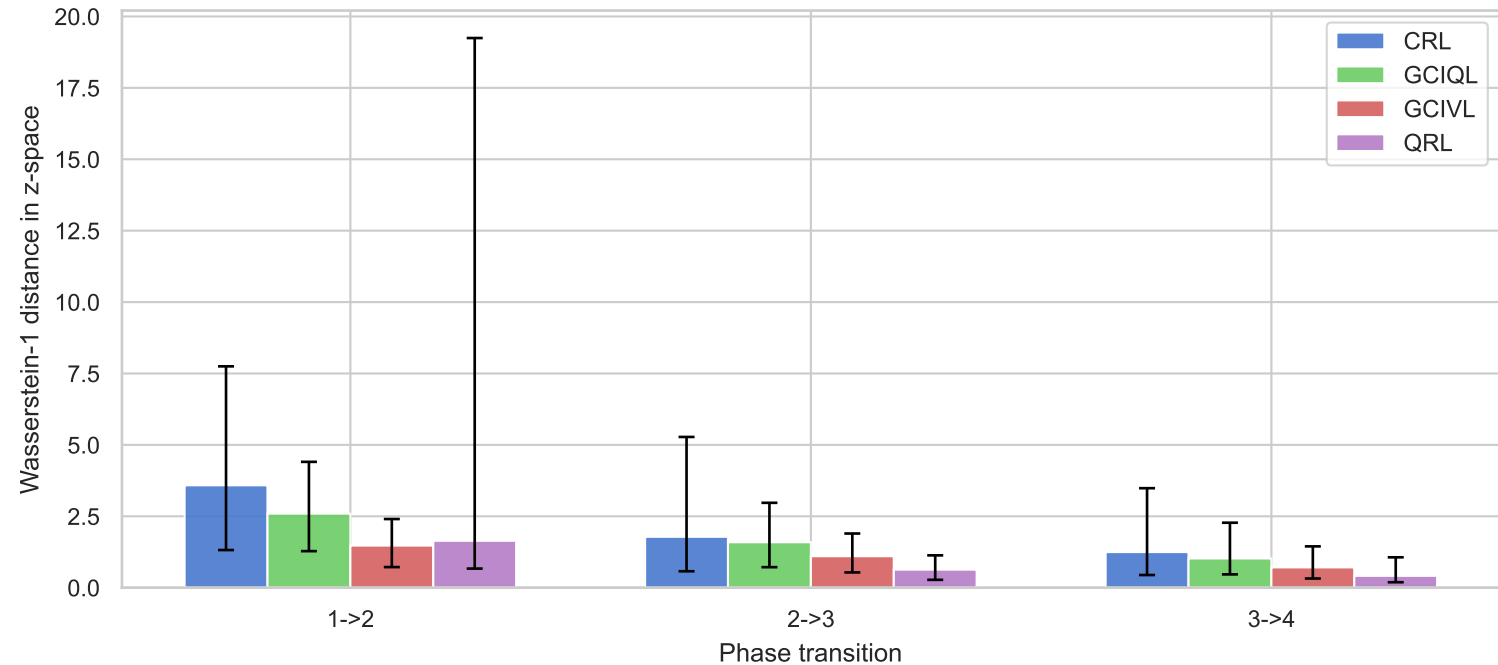
Phase-to-Phase Distribution Stability of z = \alpha \cdot A (median W1 across configs & seeds; error bars = IQR)
