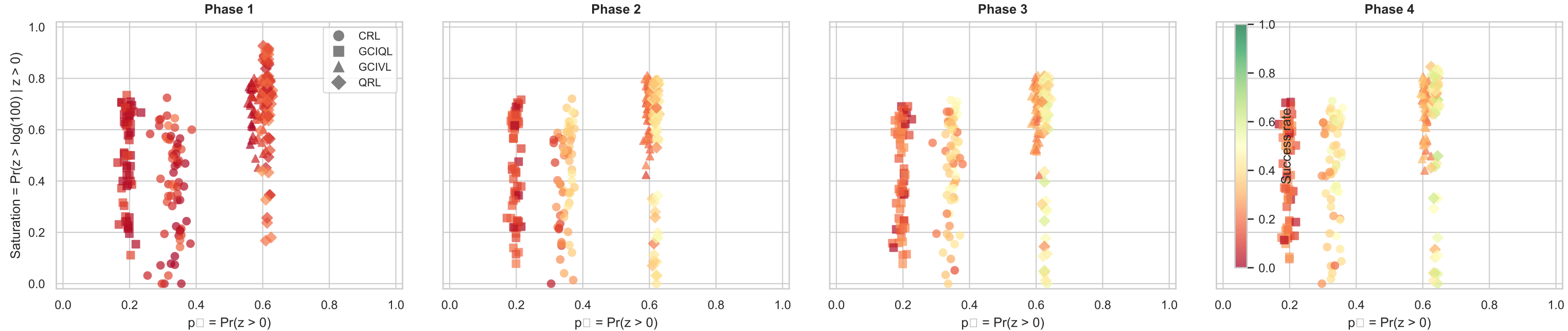
AWR 2-D Regime Map: winner fraction vs saturation, coloured by success rate (AntMaze Medium — one dot per config, median across seeds & environments)
