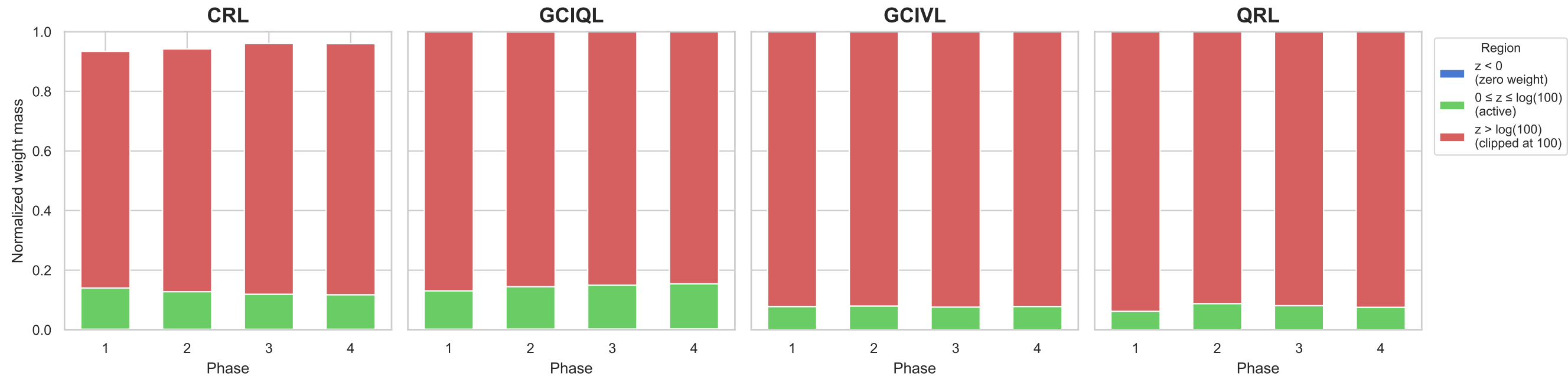
AWR Weight Mass by Region Across Training Phases (AntMaze Medium, median across configs & seeds)
