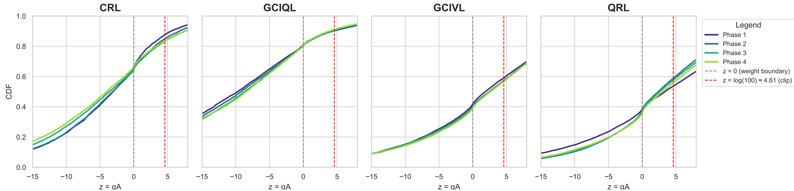
z = \alpha A CDF Across Training Phases (AntMaze Medium, median across configs, seeds & environments)
