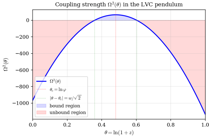
Figure 1. The coupling profile \Omega^2(\theta) defined by Axiom L4. The maximum is attained at \theta_c = \ln \varphi (red dotted line) with \Omega_0^2 = 2/w^2 . The coupling vanishes at |\theta - \theta_c| = w/\sqrt{2} (green dotted lines), separating the bound region (light blue) from the unbound region (light red).
