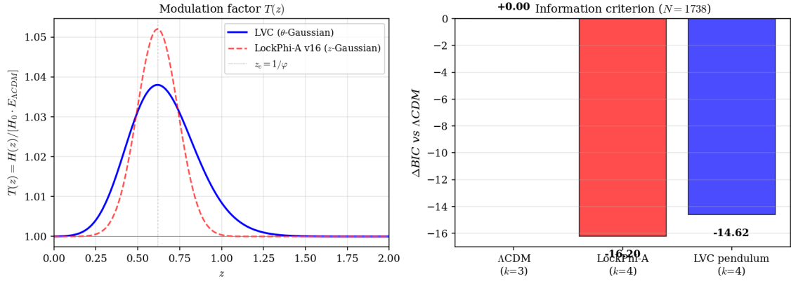
Figure 2. Left: the modulation factor T(z) of the present construction (blue, \theta -Gaussian) compared to the published Lock- \varphi -A functional form (red dashed, z -Gaussian) at A=0.052 . Right: \Delta BIC values, taken between the A=0 special case and each of the two A\neq 0 constructions, on the joint N=1738 dataset.
