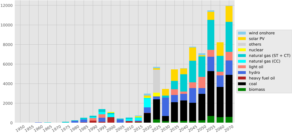
Power plant new capacity (MW)
