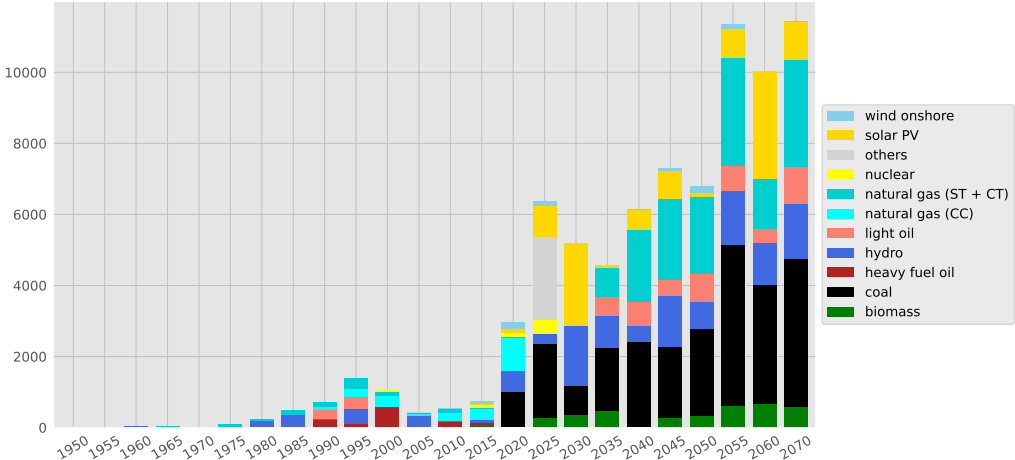
Power plant new capacity (MW)
