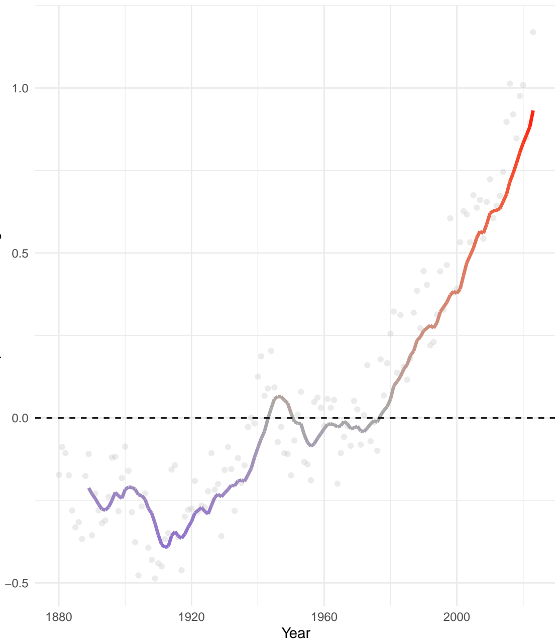
Global warming trend (1880–2023)
