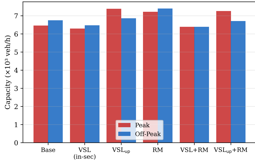
(a) Diverge instantaneous capacity
