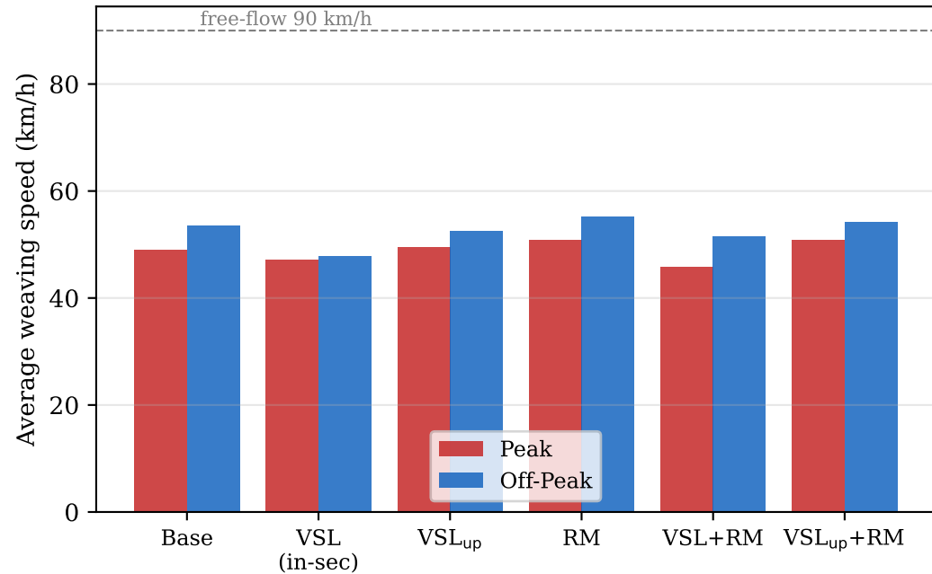
(b) Average speed on E weaving
