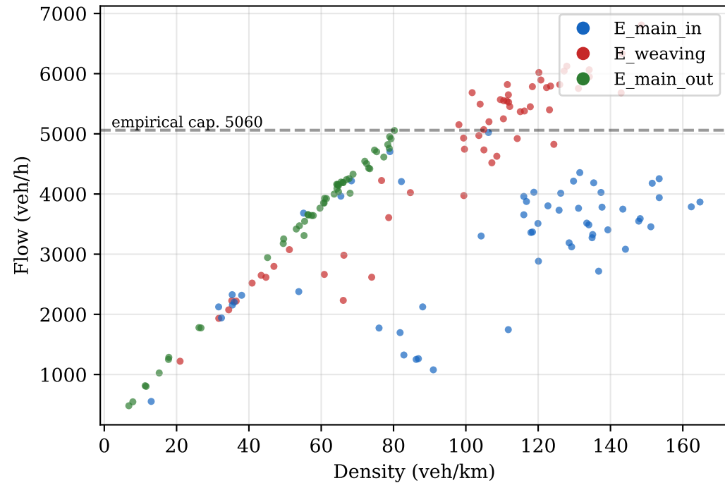
Fundamental diagram — Peak Base
