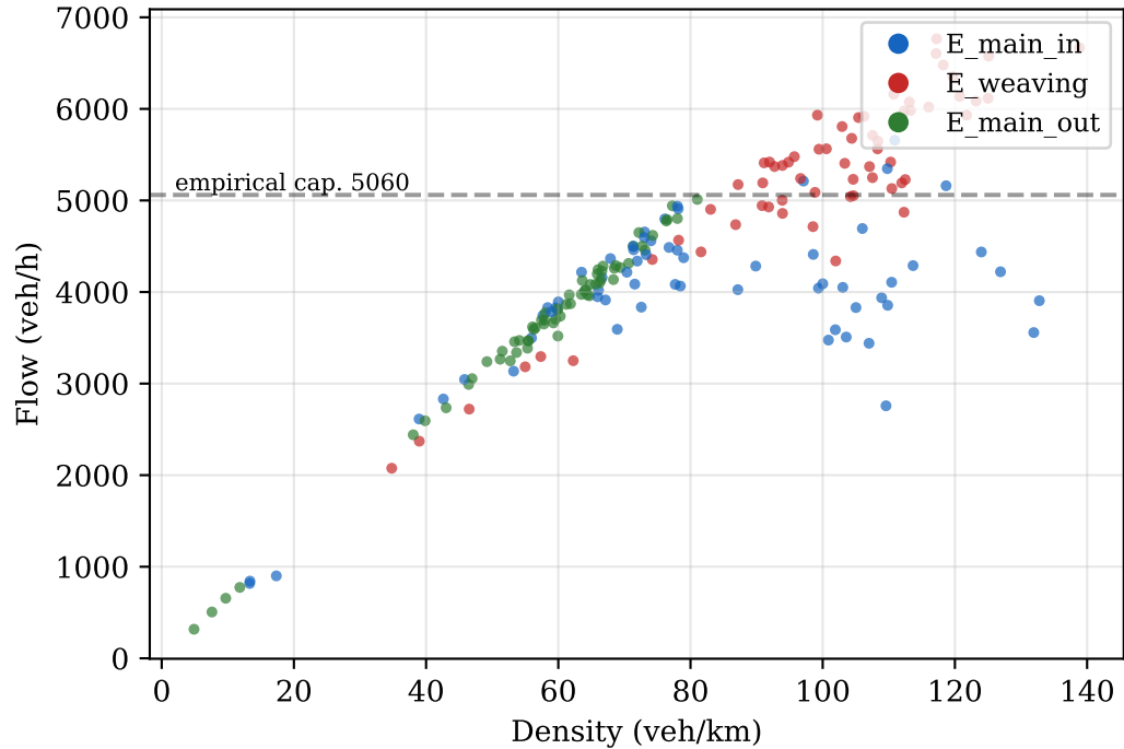
Fundamental diagram — Off-Peak Base
