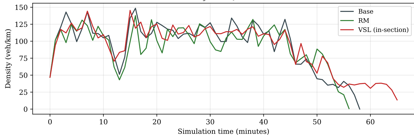
(b) E_{weaving} density time series
