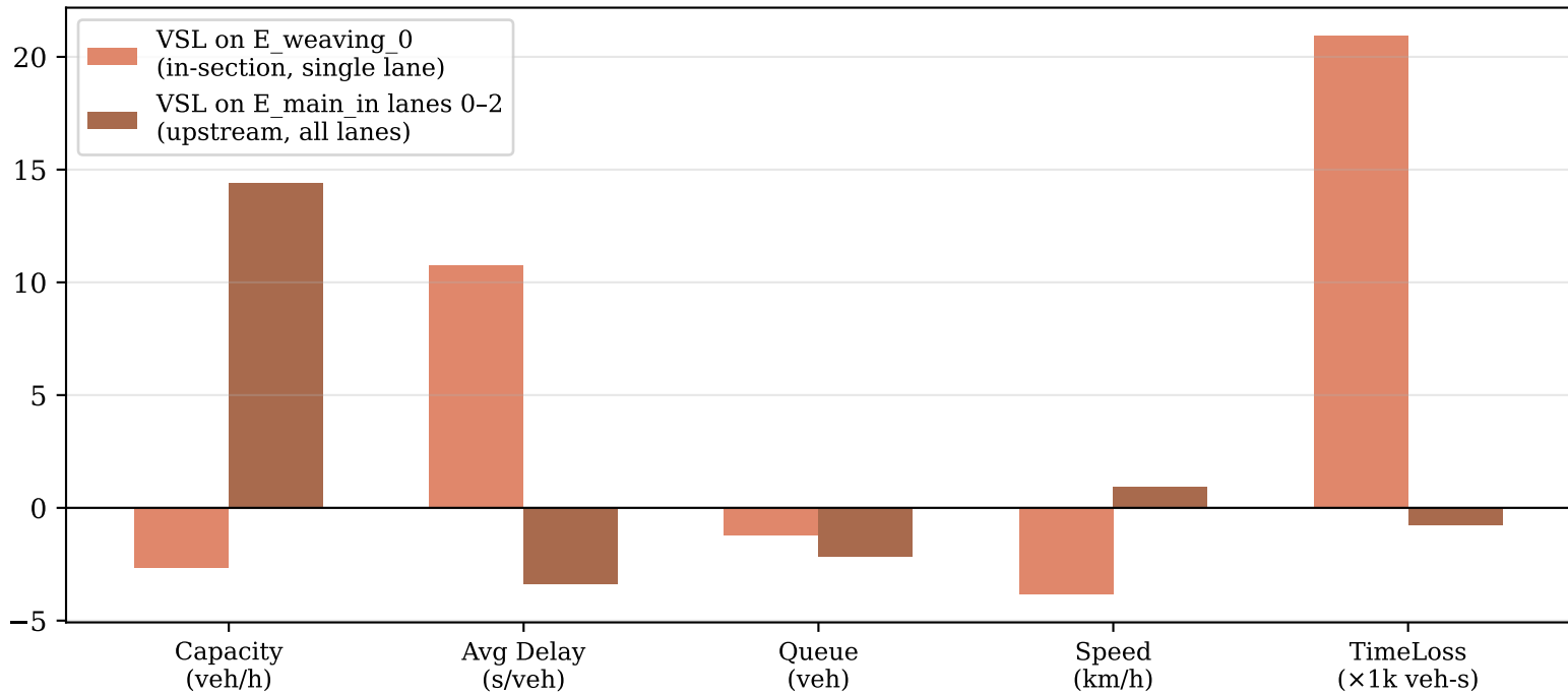
VSL placement comparison — Peak period \Delta\% relative to Base
