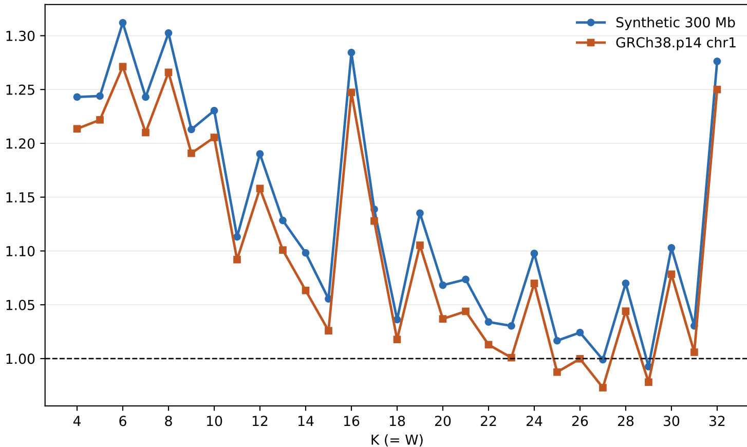
Median paired throughput ratio KSSD-Array / ntHash
