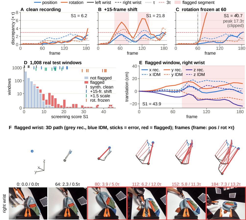
Figure 13: Data quality screening. (A–C) Per-timestep IDM-versus-recorded discrepancy for a clean recording and two corrupted controls with flagged segments shaded. (D) Screening scores over 1,008 test windows. (E) A flagged real window: recorded versus recovered right-wrist translation. (F) 3D path of the flagged wrist, recorded versus recovered with error sticks in red, and its frames.
