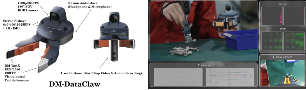
Figure 7: DM-DataClaw hardware and data collection. Device specifications and a handheld collection example, adapted from Daimon-Infinity (Daimon Robotics, 2026).
