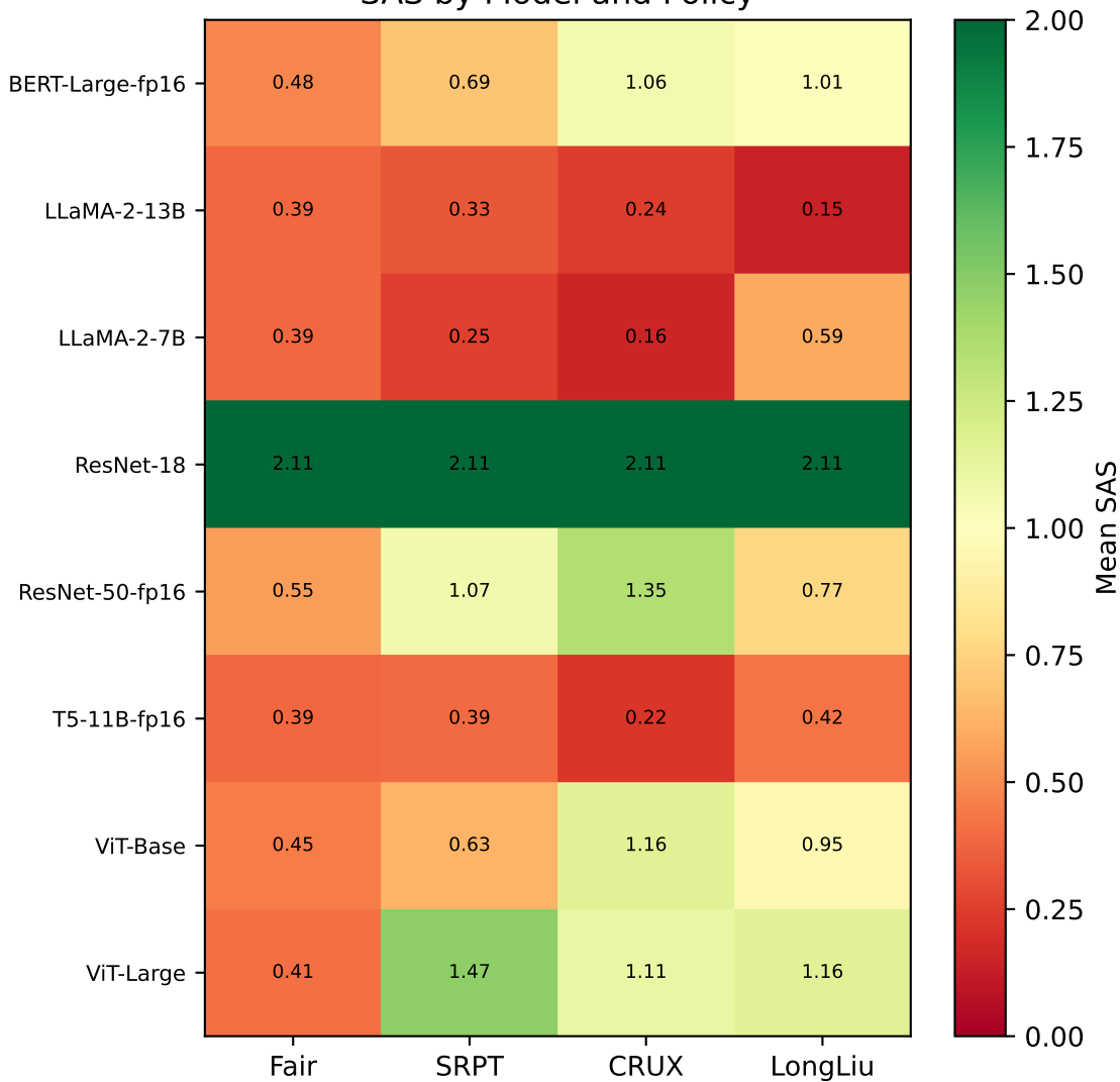
SAS by Model and Policy
