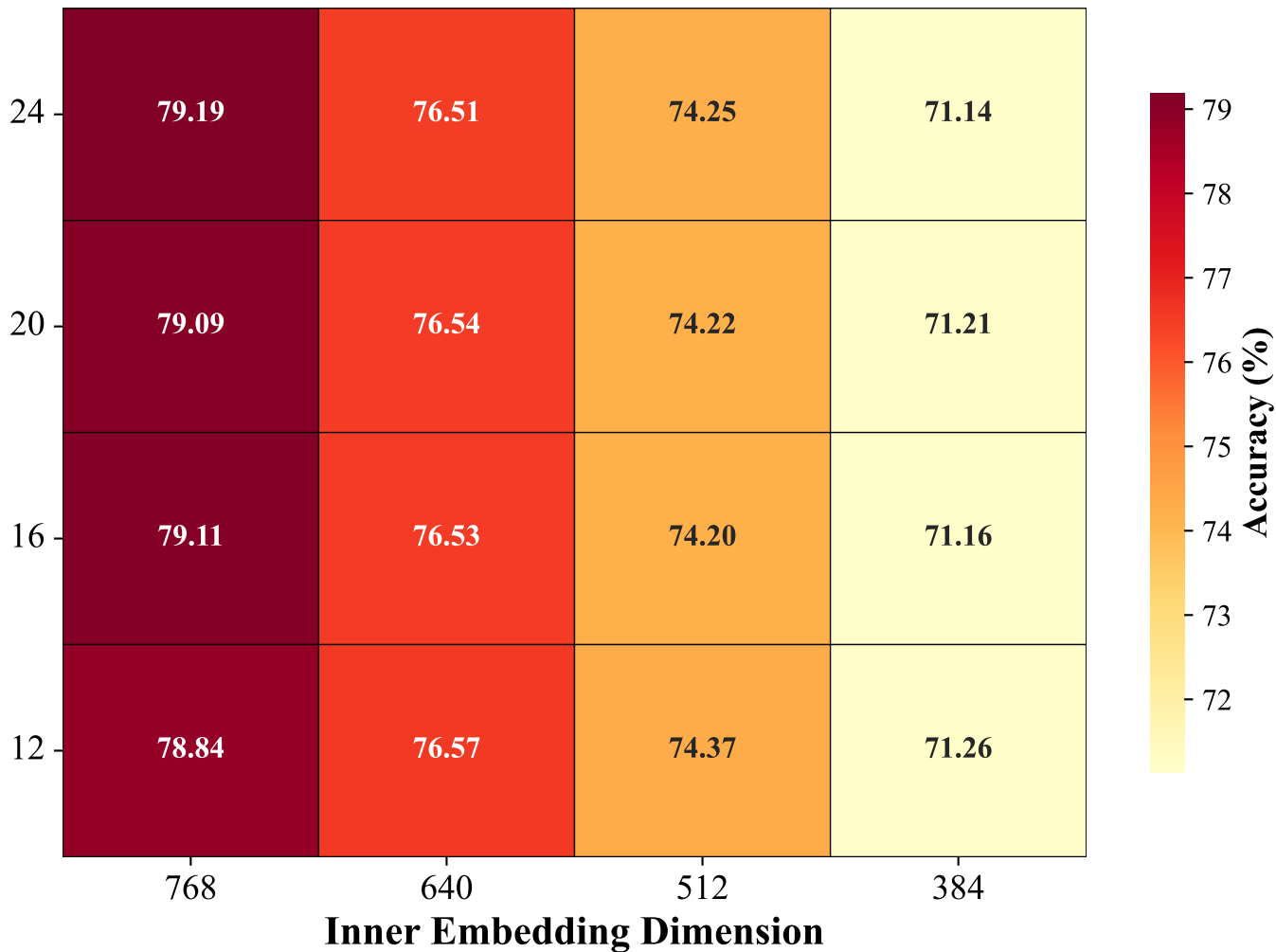
D-state vs Inner Embedding Dimension - Accuracy
