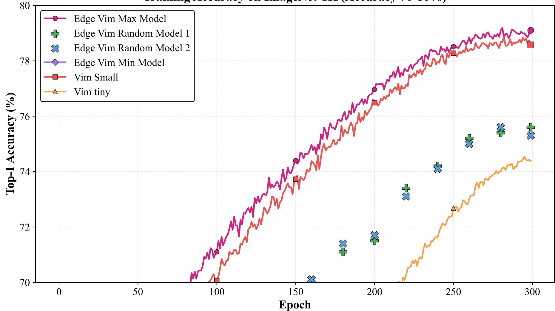
Training Accuracy on ImageNet-1K (Accuracy 70-80%)
