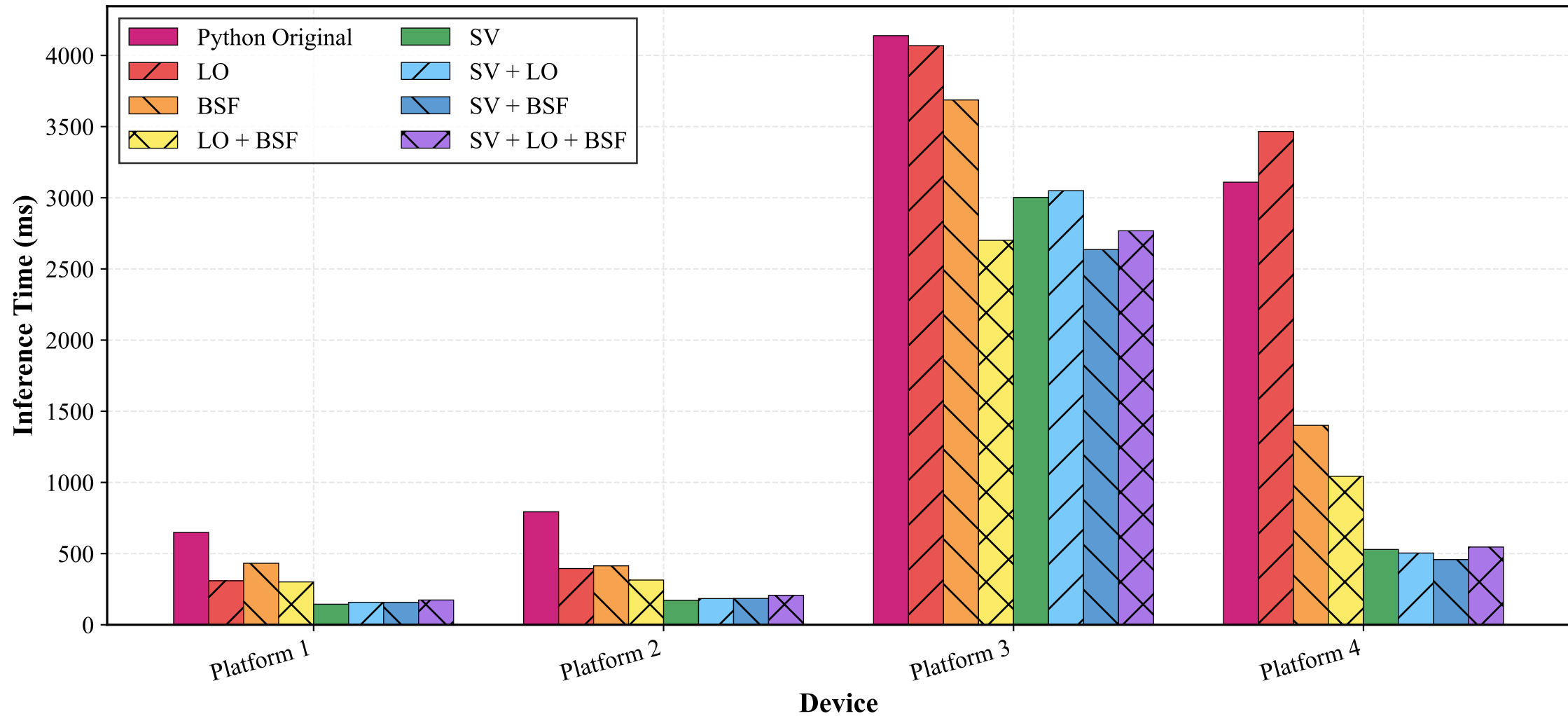
Inference Time Comparison - vim_10m
