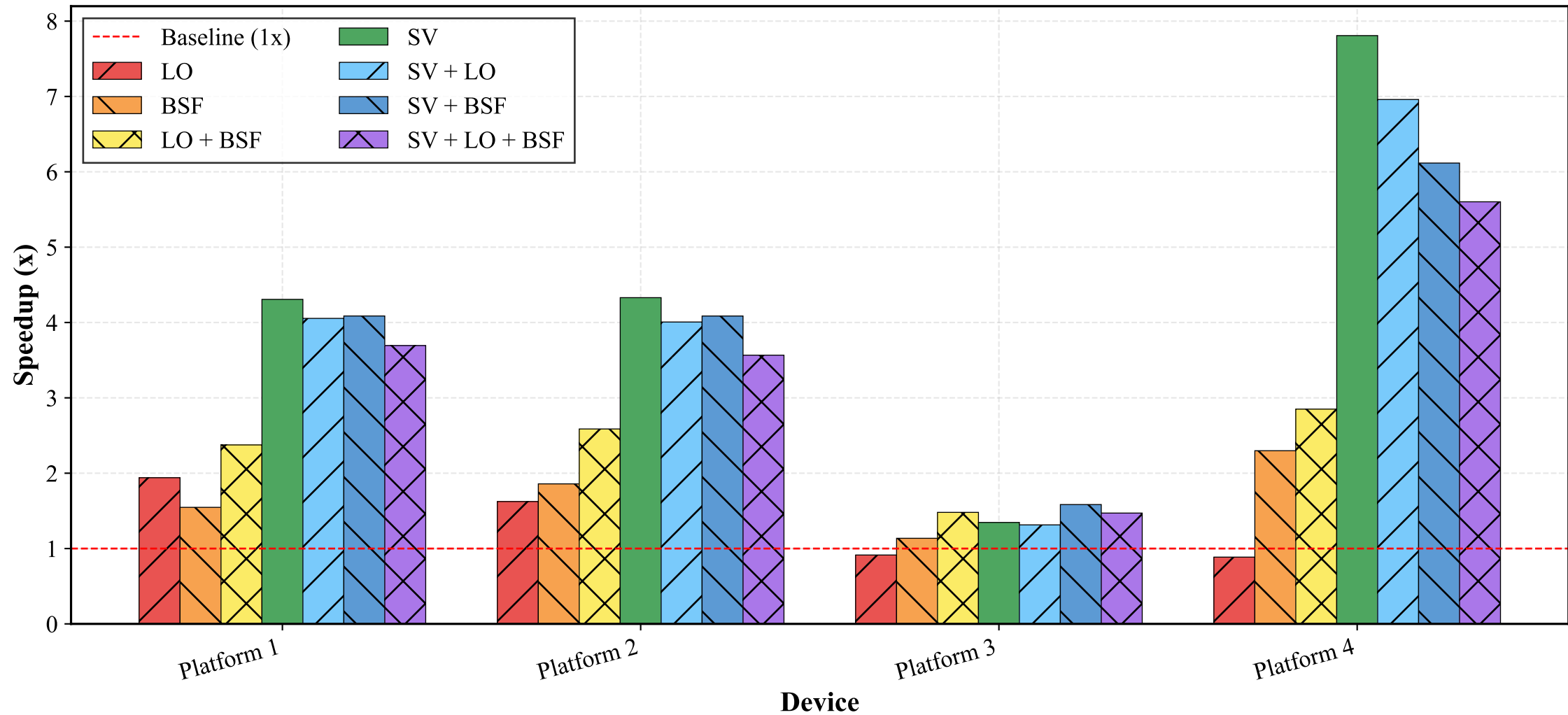
Speedup vs Python Original - vim_20m
