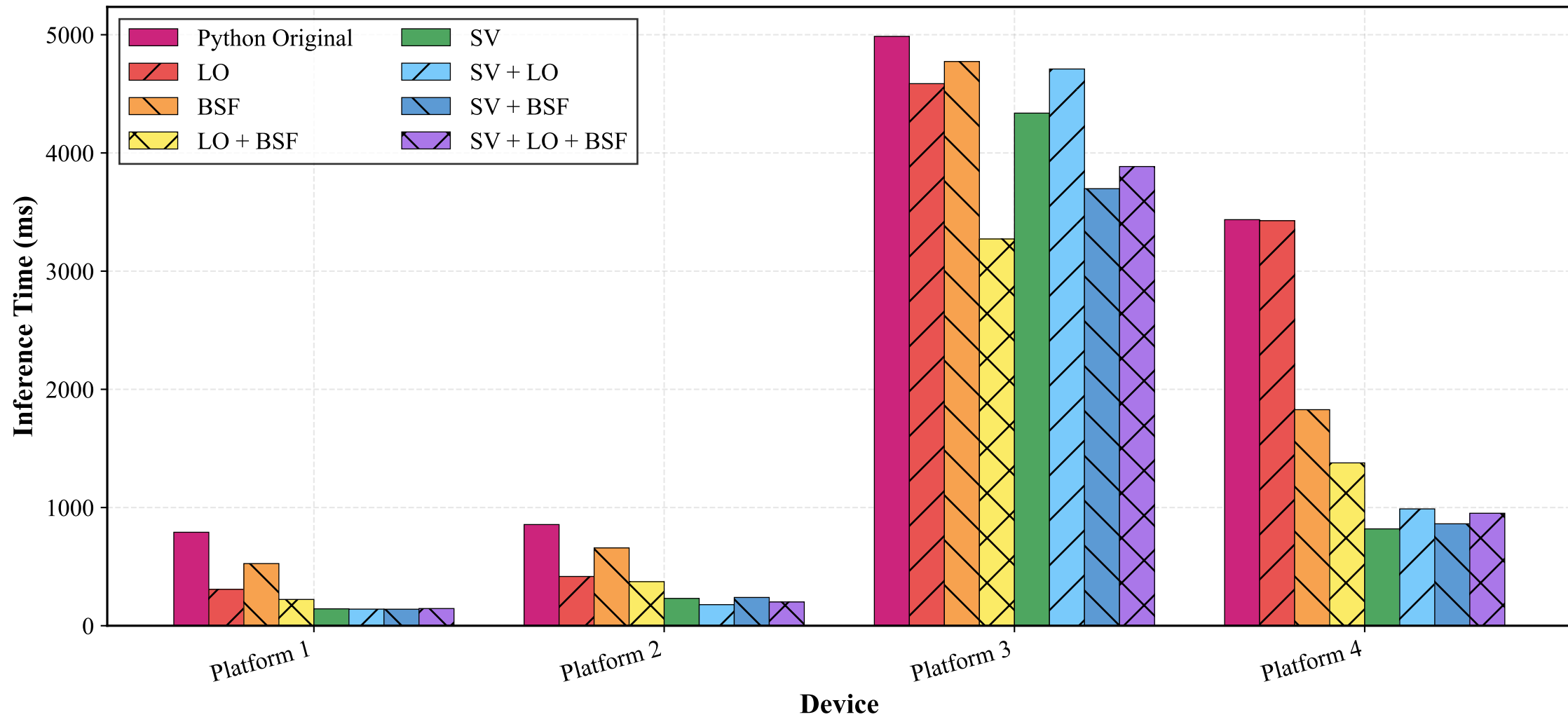
Inference Time Comparison - vim_2gflops
