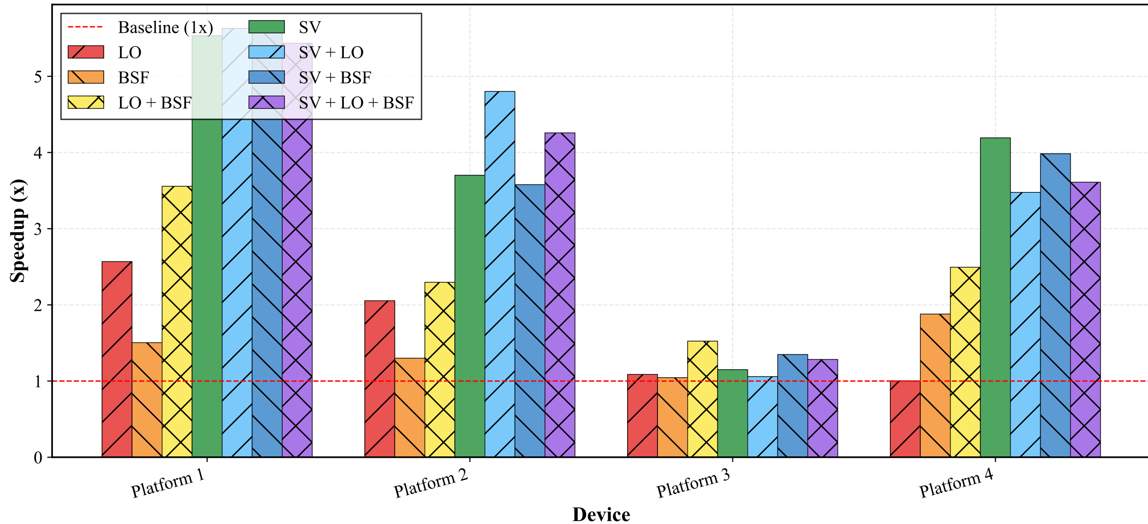
Speedup vs Python Original - vim_2gflops
