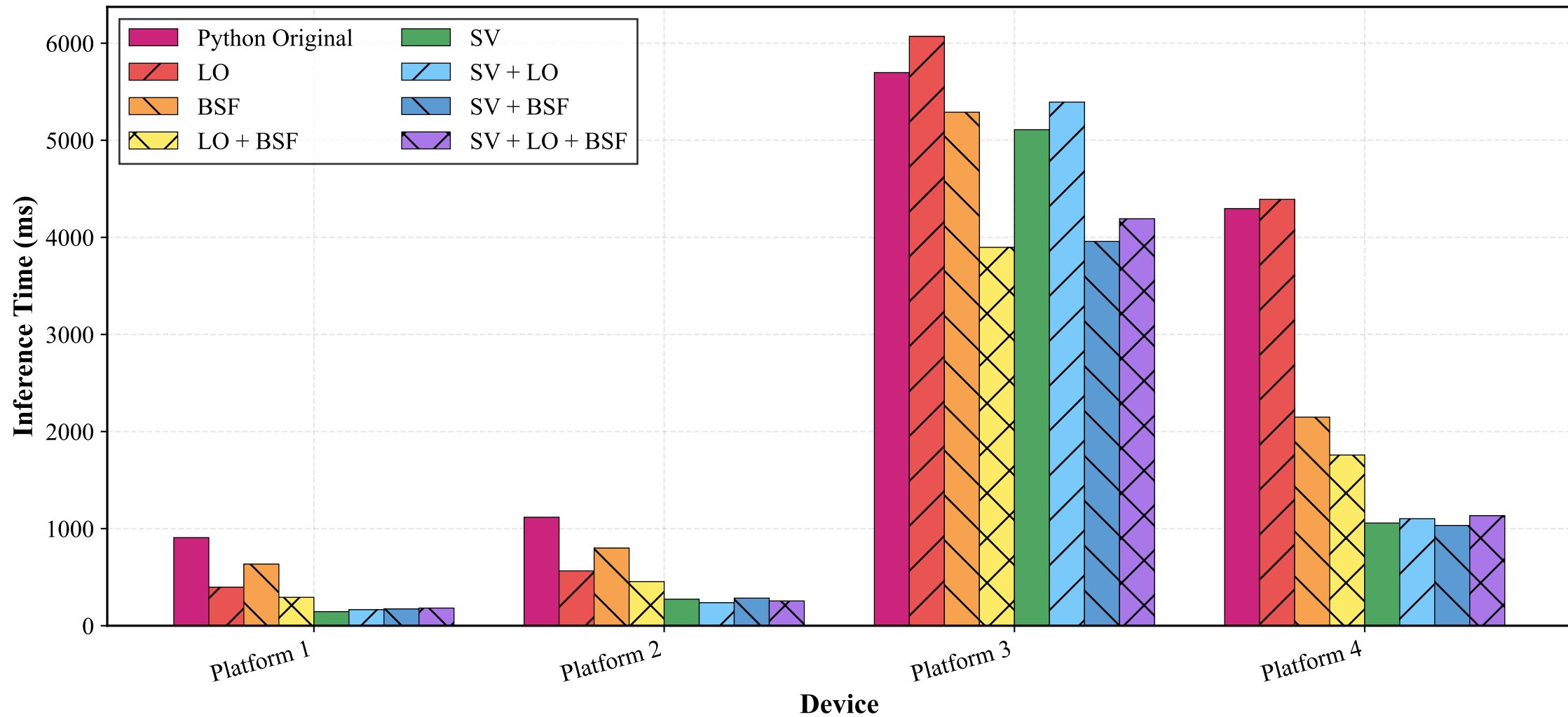
Inference Time Comparison - vim_3gflops
