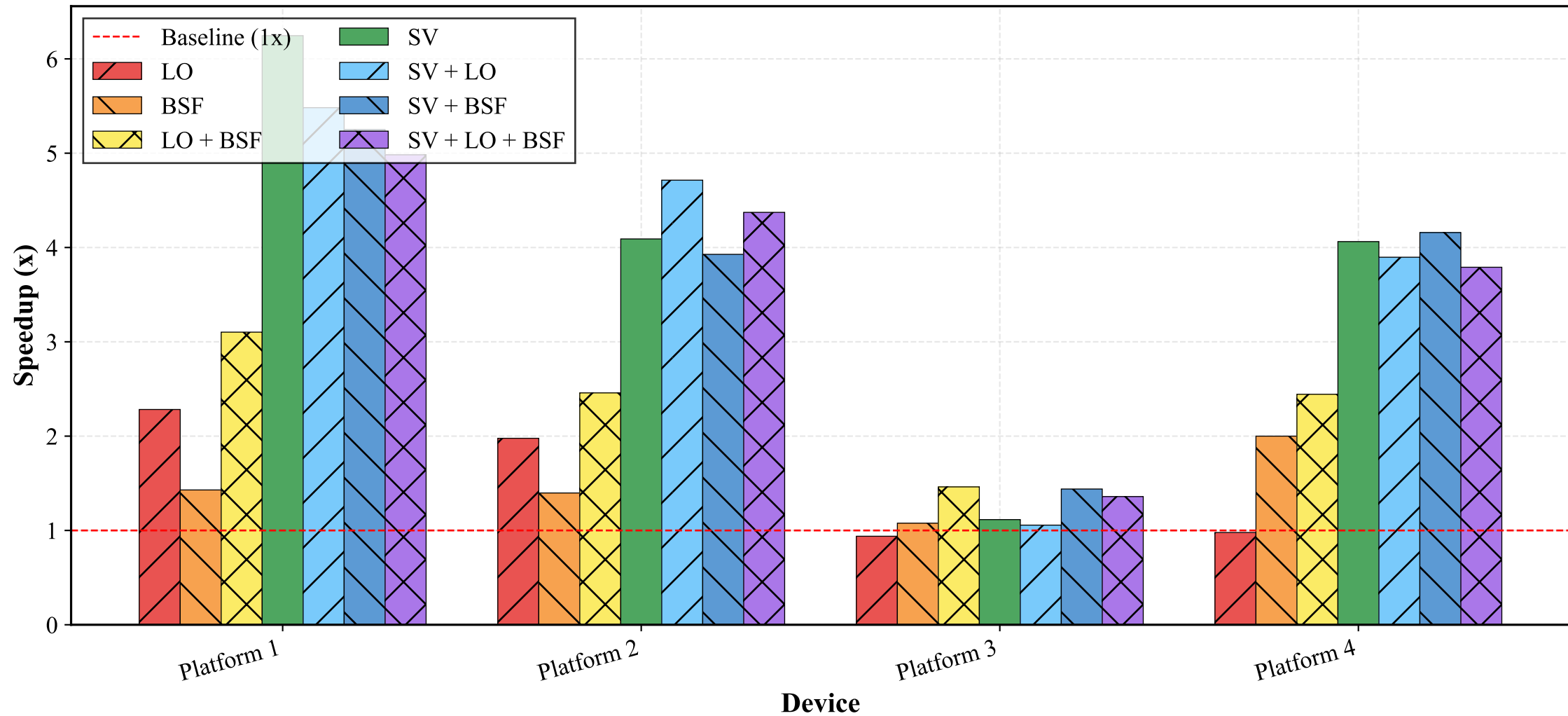
Speedup vs Python Original - vim_3gflops
