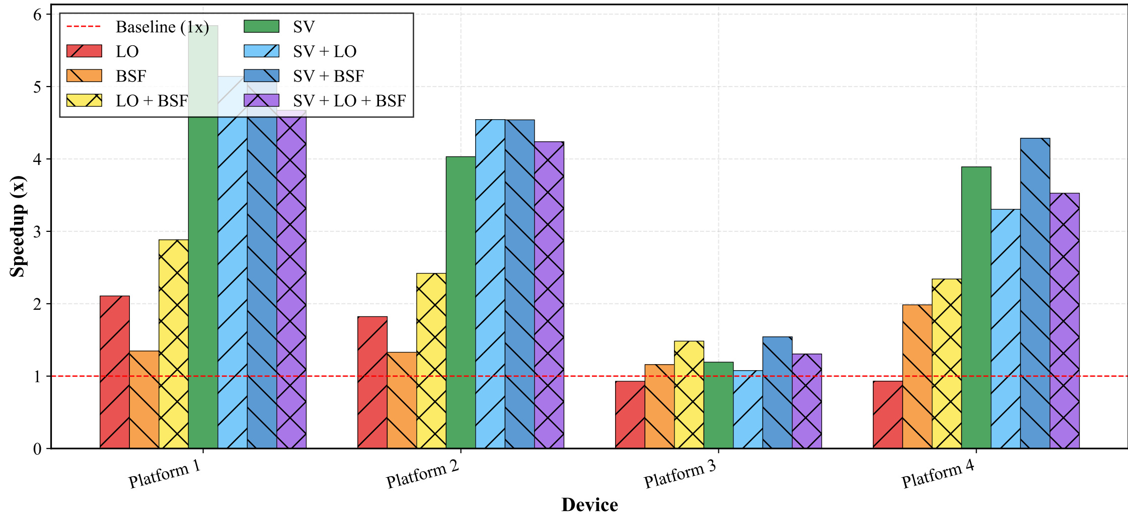
Speedup vs Python Original - vim_4gflops
