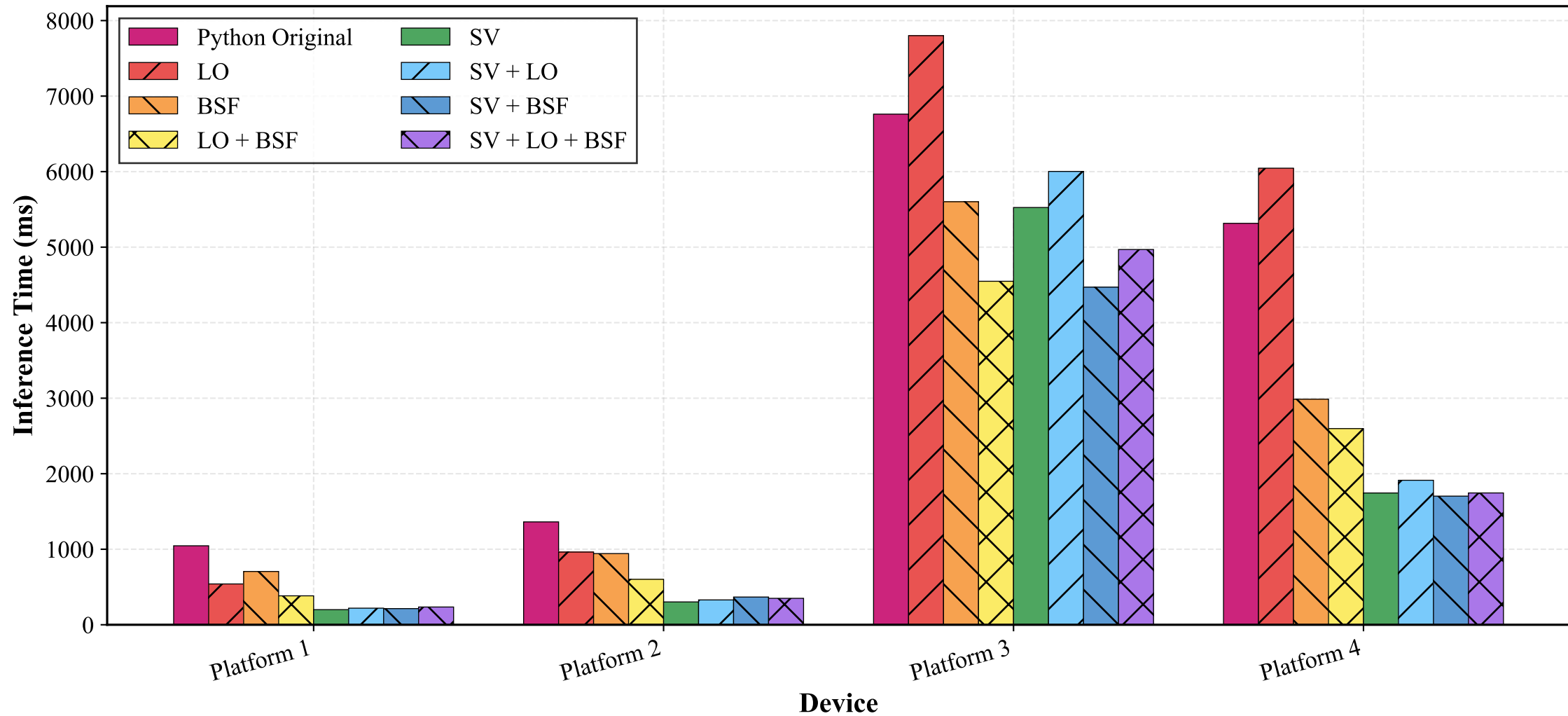
Inference Time Comparison - vim_5gflops
