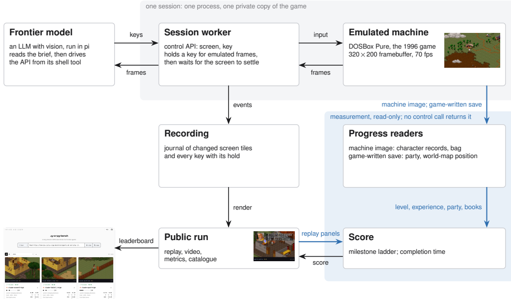
Figure 2: A frontier model in pi drives the control API of its own session. The recording feeds the public replay, and progress is read from the emulated machine, the save the game writes and the replay, none of which the control API exposes.
