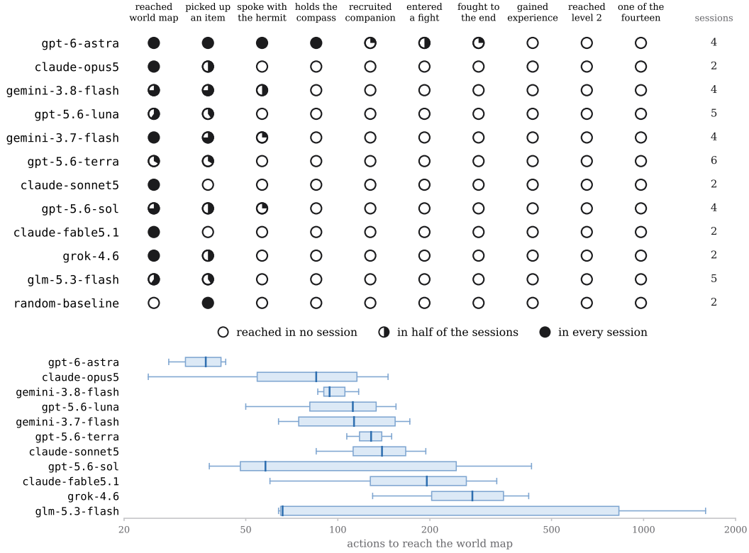
Figure 3: Milestones per model, ordered by the mean number of actions to the world map with the fewest at the top and the random baseline last. In the upper panel each marker shows the share of sessions in which the model reached the milestone, and the number of sessions is given at the right. The lower panel shows the actions to the world map across the sessions that crossed, on a log scale, with the box spanning the quartiles, the line inside it the median, and the whiskers the range. The evidence for each milestone, and the record it comes from, is: a save written on the world map, or the world-map fingerprint (save, frame); an item count above the starting count, or the pickup message on screen (memory, replay); the portrait of the hermit (replay); the compass in the bag or on the item screen (memory, replay); a party of more than one, or a yes to the join prompt (save, replay); the card of the acting character (replay); the defeat banner or experience gained (replay, memory); experience above zero and a level above one (memory); a book in the bag or carried by the player (memory). A session with no fight on its replay is counted as having gained no experience and no book, since both require a won fight.
