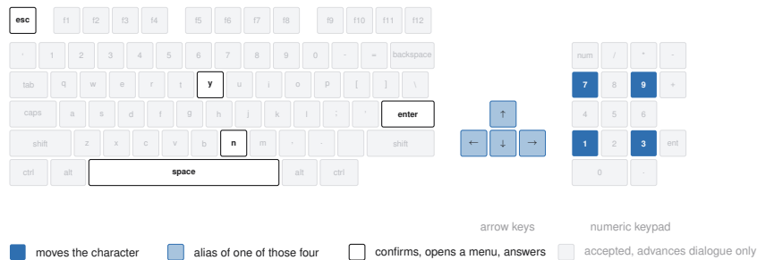
Figure 5: The keyboard the API exposes. The nine keys the game responds to outside dialogue are highlighted; the arrow keys alias the four movement keys, and any key advances a dialogue.
